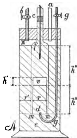
FIG. 16.—Improved Cartesian diver with double tube and influx pipe.
